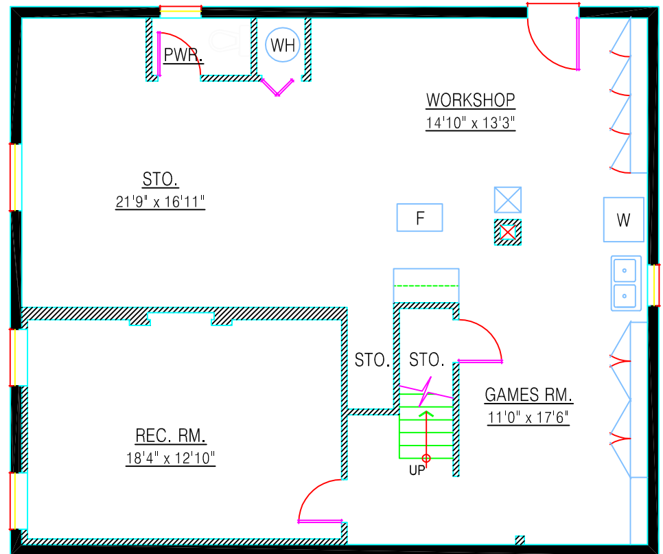
LOWER FLOOR PLAN FLOOR AREA: *1,218 sq. ft.
