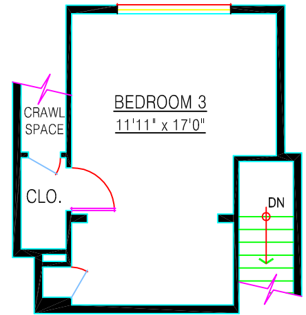
UPPER FLOOR PLAN FLOOR AREA: 236 sq. ft.
